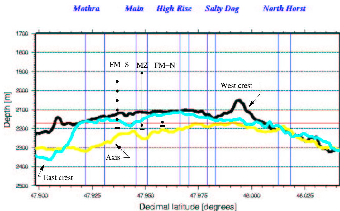
Figure 2.4: Axis-parallel bathymetric sections along the valley floor and ridge crests. Short vertical lines are 3 moorings (FM-S, MZ, and FM-N) with individual current meters (solid circles) at specific depths. Vertical lines with labels at top margin are boundaries of major vent fields. Solid horizontal line at 2170 m marks the depth of the sill near 48°N. Cross-sections are based on Hydrosweep bathymetric data (D. Kelley, 1996). Axis depths are generally deeper than the depths of the mooring bases or hydrothermal fields because the moorings and fields are often located on the shallower sides of the valley, rather than directly on the axis.
