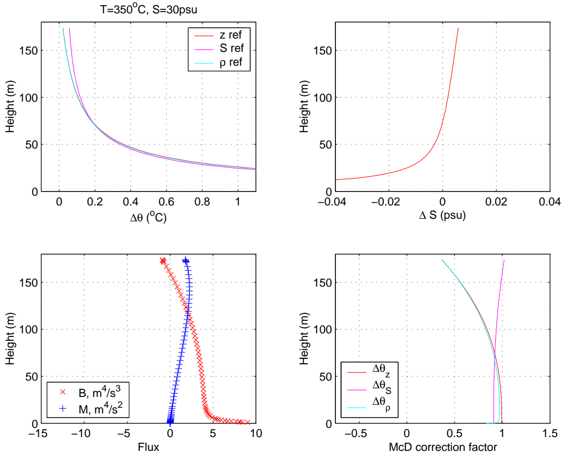
Figure 1.5: Modeled properties of a rising hydrothermal plume. Upper left panel shows profiles of temperature anomalies, referenced to depth, density, and salinity. Note that the level anomaly is slightly larger than the isopycnal anomaly over this depth range; they are distinct immediately above the source at very large anomaly values (not shown). Upper right panel shows profile of level salinity anomaly. Lower left panel illustrates how buoyancy flux, B and momentum flux M change as the plume rises to its maximum height. Lower right panel depicts the profile of McD factor, the ratio of vertical to source heat flux, for different temperature anomalies used to calculate the vertical flux.
