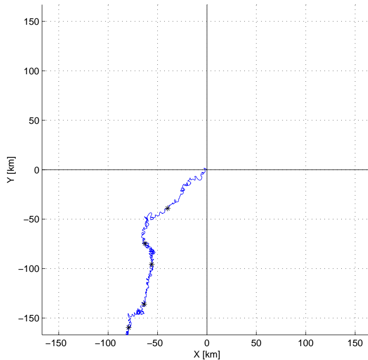
Figure 2.10: Progressive vector diagram for the 1995 current meter (300 mab, 1900 m) near the northeast corner of the MEF field. The mean flow for this 52.5 day record is 4.10 cm/s at 206^\circ . Black asterisks symbolize 10 day intervals.
