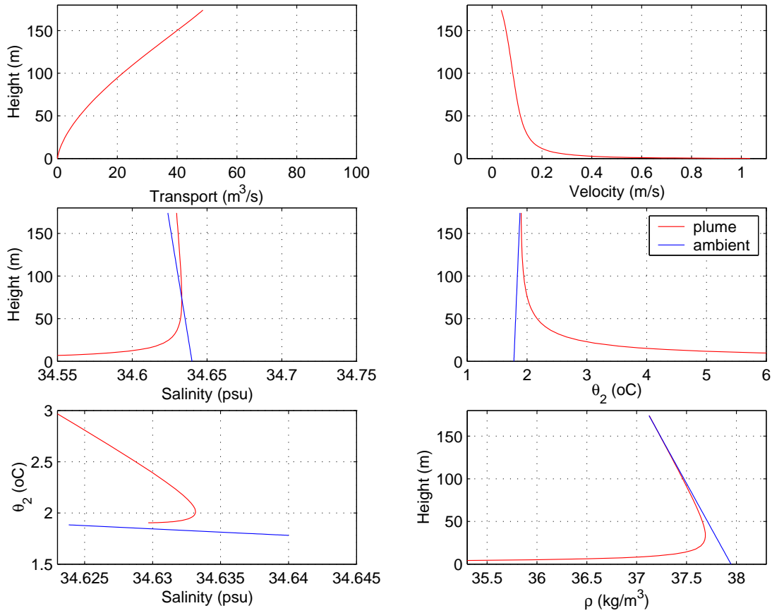
Figure 1.4: Modeled plume properties for a source with \theta_o = 350^\circ\text{C} and S_o = 30 psu, and ambient \theta and S profiles typical of the deep northeast Pacific. All panels are depth profiles of ambient and in-plume conditions except the lower left \theta - S diagram. Proceeding counter-clockwise from lower right panel, profiles are of density, potential temperature, vertical velocity, vertical transport, and salinity.
