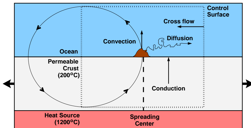
Figure 1.1: A schematic depiction of processes that transfer energy between the mantle, crust, and ocean at the axis of a spreading center. In assessing the heat flux associated with each process, the scale of the control surface over which a flux is measured will be different.
