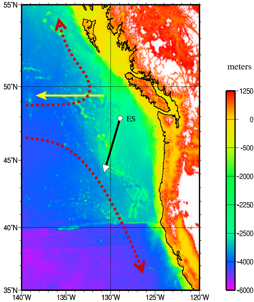
Figure 2.9: Bathymetric map of the northeast Pacific ocean off the coast of Washington (SMITH and SANDWELL 1997) with regional mean currents overlain. Dashed arrows indicate bifurcating surface currents. Solid arrow shows westward Subarctic counter-current on surface. Solid arrow indicates long-term mean flow over the Endeavour segment near 2000 m, a typical plume equilibration depth (denoted by white diamond).
