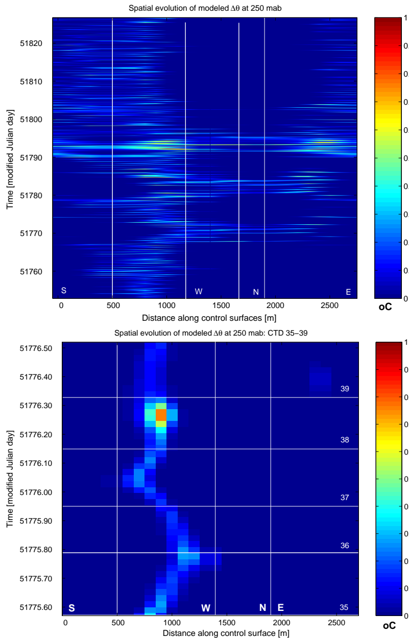
Figure 4.10: Time series of \Delta\theta on the 4 MEF control surfaces, based on the current record from FM-S200. Vertical axis is time in days with model time steps of 1/2 hr; horizontal axis is distance along successive control surfaces. Upper panel shows the full current meter record (Flow Mow cruise period is MJD 51760–51777); lower panel shows only the period of the circumnavigation stations (MJD 51775.60–51776.52). Horizontal white lines mark the beginnings of CTD stations 35–39, while vertical white lines represent boundaries between the 4 control surfaces (folded flat as in Figure 4.4 and labeled with a letter denoting cardinal direction).
