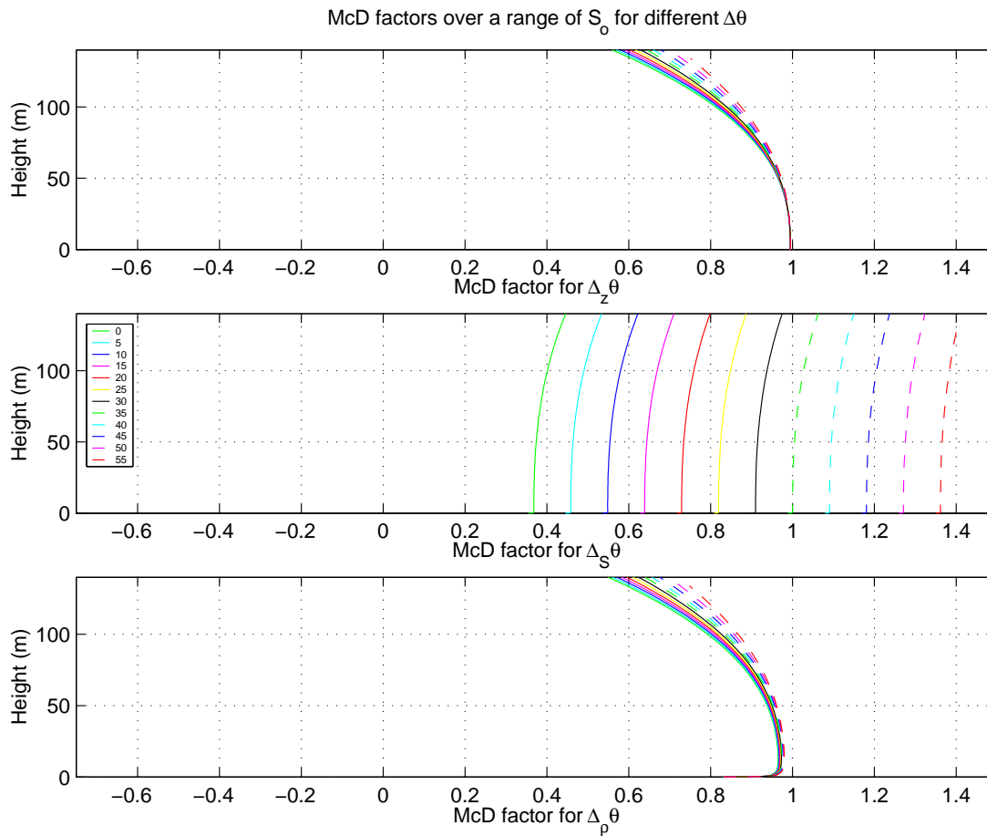
Figure 1.6: Correction factors for modeled vertical heat flux calculated with different types of temperature anomalies. Upper to lower panels show correction profiles for level, isohaline, and isopycnal temperature anomalies, respectively. Note that profiles are truncated at 130 meters above bottom in order to emphasize the evolution of properties within the first 100 m of rise.
