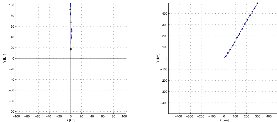
Figure 2.13: Progressive vector diagrams for axial valley currents measured at the central mooring in 1995 (MZ95, 25 mab, 2175 m) and the northern mooring in 2000 (FM-N, 15 mab, 2162 m). Mean flow is 4.74 cm/s at 31^\circ for MZ95, and 2.29 cm/s at 0^\circ for FM-N15. Relative to the multidirectional flow above the ridge, the mean flow in the valley at these meters is rectilinear and consistently northward. Black asterisks are 10 day intervals. Note that domain and range are different between plots.
