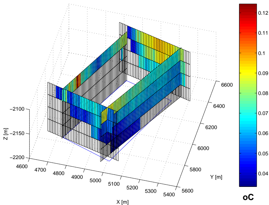
Figure 3.5: \Delta\theta distribution on all 4 side surfaces of the MEF control volume, acquired within a 15.4 hr period during ABE dive 50. Observations are projected on to vertical planes aligned with the mean track of ABE on each side, rather than on to the control surfaces. Coordinates are relative to the Alvin origin.
