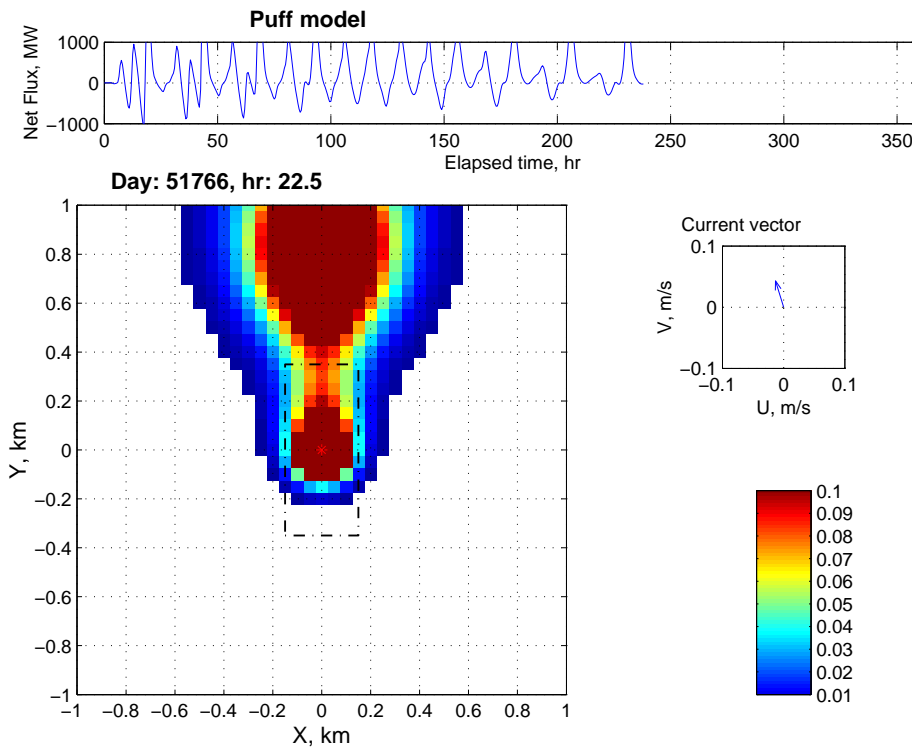
Figure 3.8: A single frame from a puff model animation showing a plan view of a thermal plume extending northward from the MEF (dashed black rectangle). In this snapshot, 240 hr into a 360 hr simulation, the puffs are advected by idealized flow (a 1 cm/s mean added to an oscillation derived by H. Mofjeld through harmonic analysis of the record from the MZ25 current meter; c.f. Figure 2.18.) and the source flux is constant (300 MW). Smaller panels show: time series of instantaneous net flux through the MEF perimeter (top); half-hourly current vector (middle right) with reference arrow indicating true north; and color bar with temperature anomaly units in ^{\circ}\text{C} (lower right). At this moment in the simulation, despite the substantial anomalies on the north surface, the net flux has dropped to zero because the flow is near zero. Animations of the puff model and Bill Lavelle's diffuse plume model are provided as supplementary material: website: econsience.org/scott/pubs/thesis/animations.html
