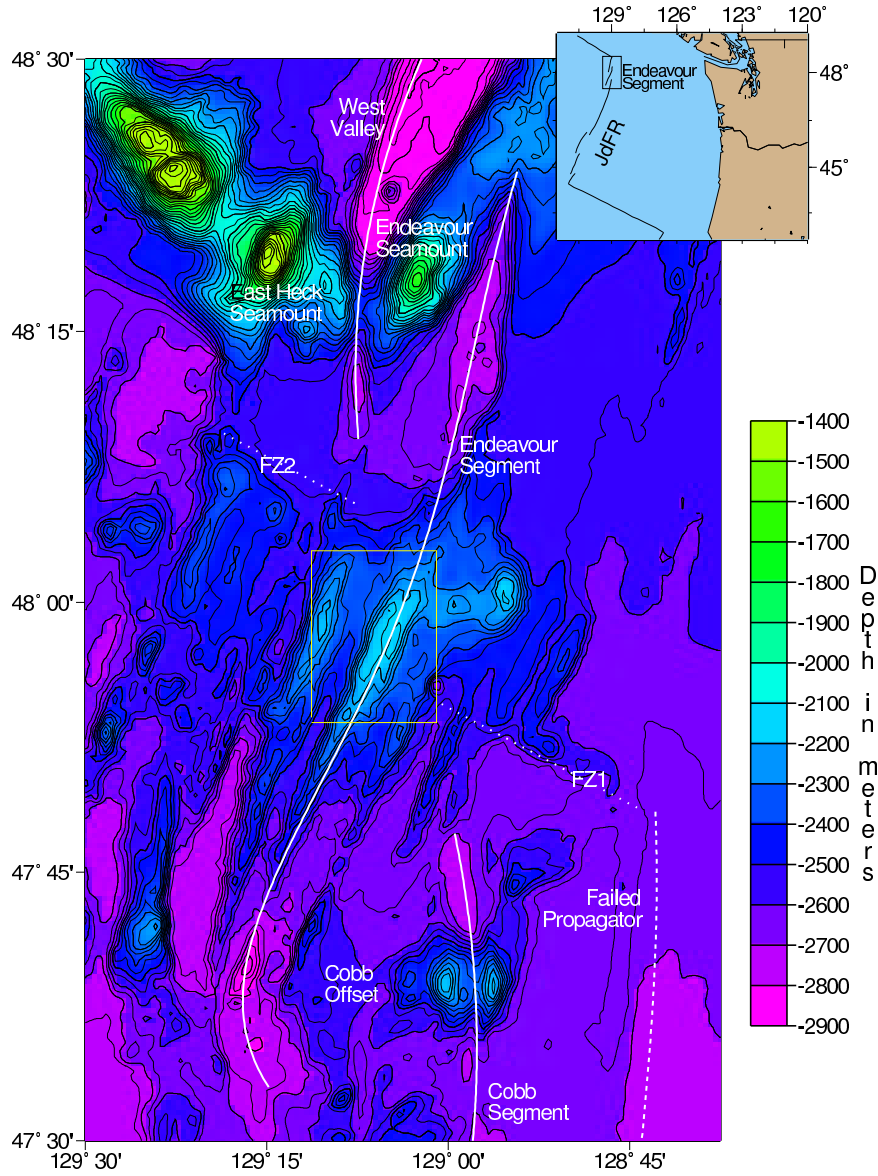
Figure 2.3: Sea Beam bathymetric map of prominent topography in the vicinity of the Endeavour segment. Contour interval is 100 m. Solid lines are inferred tectonic boundaries. Dotted lines are hypothetical boundaries and fracture zones (FZ), suggested by microearthquake distributions. Figure courtesy S. Archer and V. Bhat.
