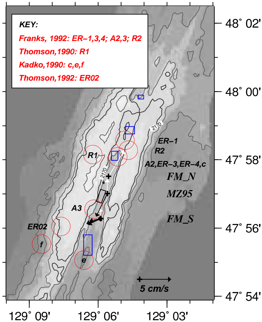
Figure 2.8: Location of current meter moorings, both historic and utilized in the planning or conduction of the Flow Mow field program. The northern and southern Flow Mow moorings are FM-N, and FM-S; the 1995 Mixing Zephyrs mooring is MZ95. Historic moorings are located with large open circles to emphasize the imprecision of Loran-C coordinates; adjacent or central labels are consistent with past studies listed in the key. For each meter on the FM and MZ moorings, the average flow observed over the full record is indicated with a vector. White vectors indicate flow within the axial valley (meter located deeper than 2100 m); black vectors show flow at or above the ridge crests (shallower than 2100 m). A 5 cm/s reference vector is provided in the lower right hand corner. To minimize clutter only major hydrothermal fields are delineated.
