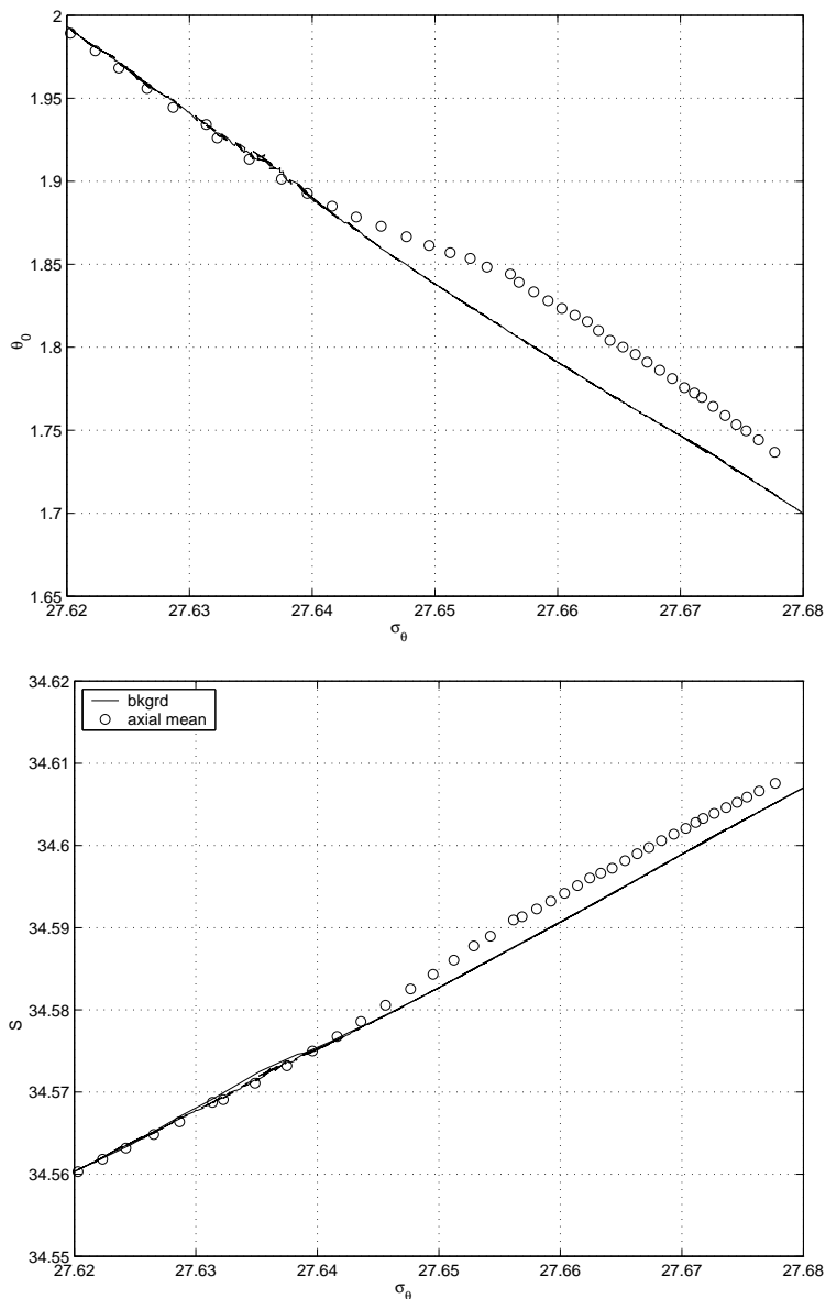
Figure 2.19: \sigma_\theta versus mean \theta and S for Flow Mow background and axial CTD stations. The solid line represents the background data (from both stations and both pairs of sensors), while the open circles represent 10 m depth-binned averages of data (from the second pair of C/T sensors only, Figure 2.7) at stations located along the ridge axis. Specific station numbers included in these averages are: 3–8, 10, 12–14, 16, 17, 19, 20, 21, 23, 24, 27, 28, 33, and 34 (see Flow Mow CTD web site, www2.ocean.washington.edu/flowmow/ecr/ctd for details and data).
