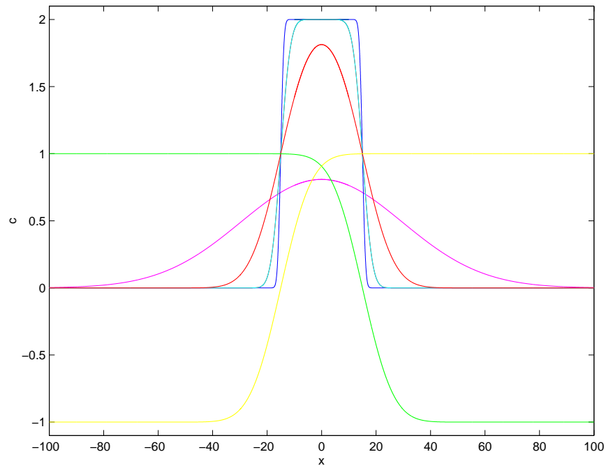
Figure 3.7: Examples of concentration c profiles for an individual puff as a function of distance x . The distribution in each dimension is governed by the sum of 2 error functions; the sum of the 2 error functions that intercept c = \pm 1 describes the initial top hat profile, but as the error functions evolve with time, their sum yields increasingly broad Gaussian curves. In this example, the initial half-width r = 15 m.
