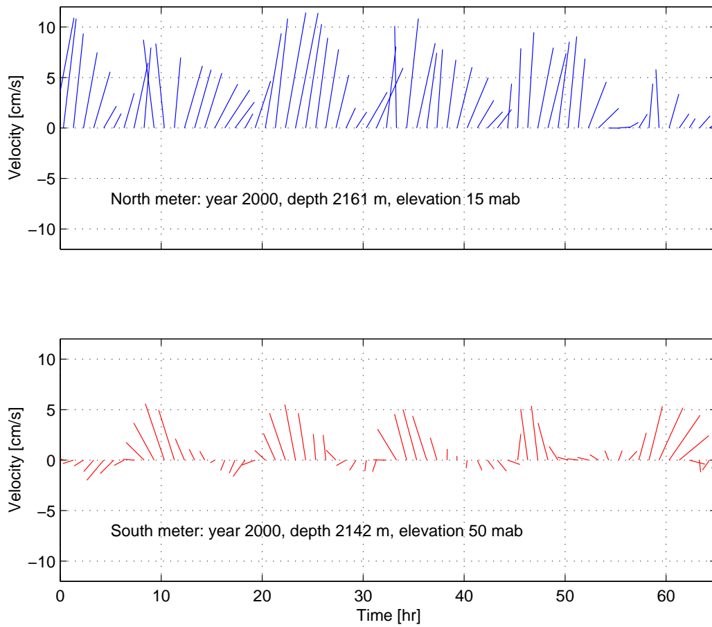
Figure 2.15: A characteristic 65 hr time series of hourly-mean currents within the axial valley north (top) and south (bottom) of the MEF. True north is up.
