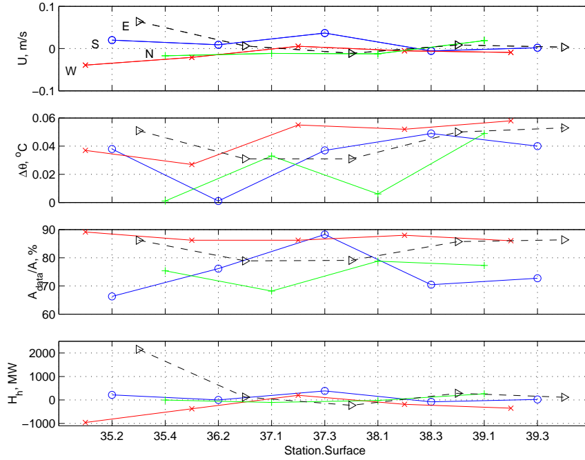
Figure 4.6: Time series of observations made on individual side surfaces during circumnavigation of the upper control volume (Stations 35–39). Panels (top to bottom) portray: mean orthogonal u ; mean \Delta\theta ; data coverage as percent of total surface area; and heat flux (positive outward). Lines connect sequential observations made on the same side surface and are labeled only in upper panel: circles=south; x=west; +=north; triangles=east. Horizontal axis labels indicate the station number and surface number during that station, separated by a decimal point (station.surface).
