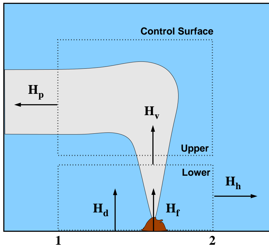
Figure 1.3: A field-scale control volume divided vertically at a height where rising plumes have a size and signal strength that is optimal for quantifying H_v , the net vertical flux through the top of the lower control volume. H_h and H_p are the net horizontal fluxes through the side surfaces of the lower and upper control volumes, respectively. H_f and H_d represent the source heat fluxes from focused and diffuse vents. Vertical surfaces are labeled 1 and 2; remaining side surfaces (3 & 4, not depicted) are parallel to the mean flow.
