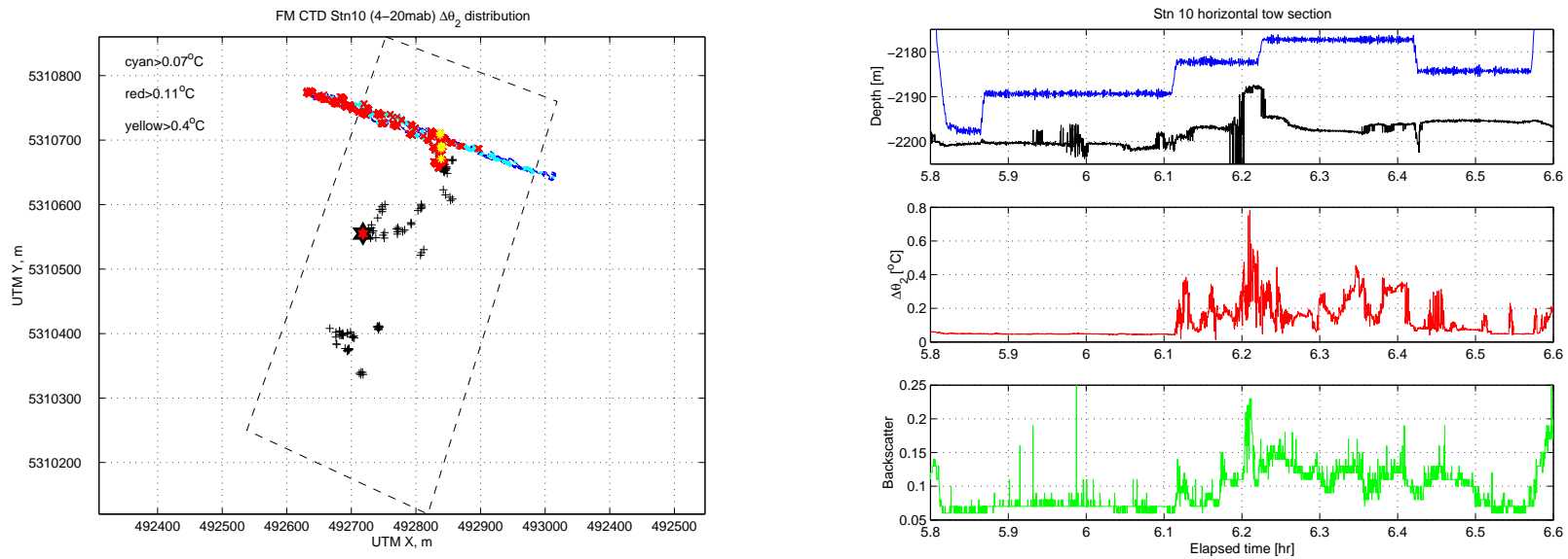
Figure 2.26: Location map and time series from horizontal tow through buoyant plumes during CTD 10 which proceeded from north to south. Left panel symbols: dashed line is MEF control volume perimeter; each + is a known individual high B source; colored x and * symbols indicate thresholds of \Delta\theta annotated in upper left corner. Right panels shows time series of depth and bottom traces (upper), \Delta\theta (middle), and backscatter (lower). Bottom depth values are sum of CTD pressure depth and altimeter reading.
