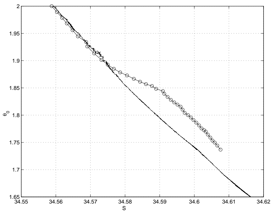
Figure 2.20: The depth-binned average \theta and S from background (solid line) and axial (open circle) stations, over the depth range common to all stations.
