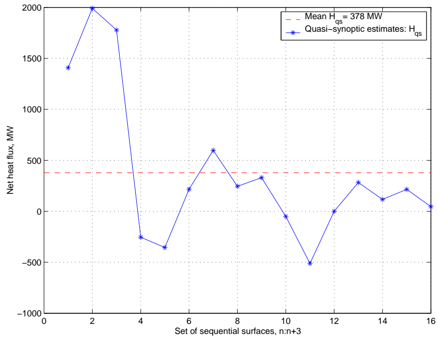
Figure 4.7: Series of 16 estimates of the “quasi-synoptic” net horizontal heat flux H_{qs} through the upper MEF control volume. The mean magnitude \overline{H_{qs}} , is overlain for reference. Each estimate was derived by summing a set of 4 sequential surfaces from the 19 total observed surfaces (see Equation 4.3). The mean, standard error of the mean, and standard deviation of the quasi-synoptic estimates are 378, 182, and \pm 730 MW, respectively.
