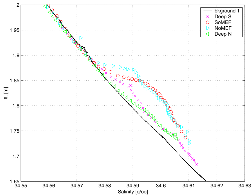
Figure 2.22: \theta - S profiles based on data, averaged in 10 m depth bins, from Flow Mow stations grouped geographically and labeled as in Figure 2.21.
