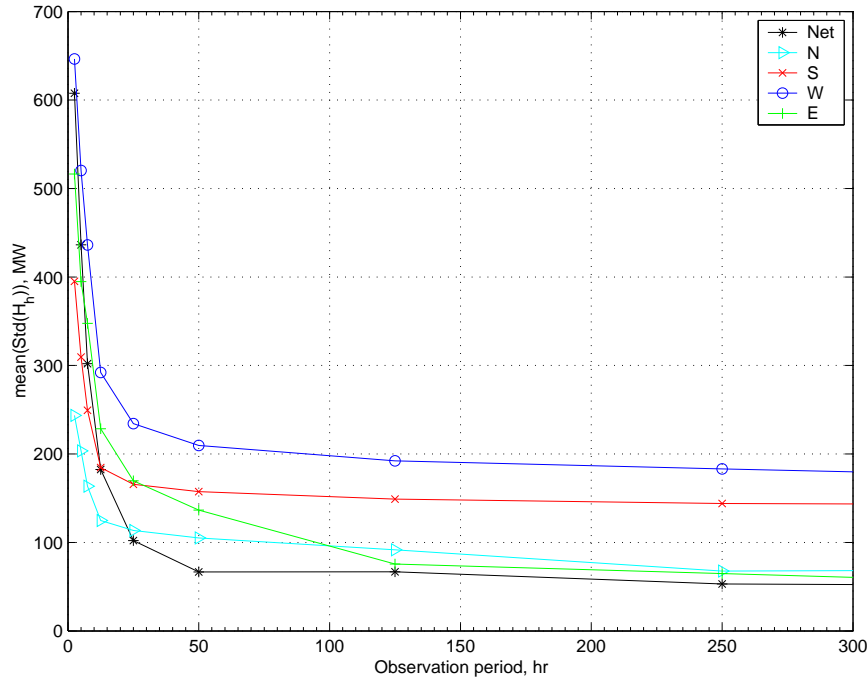
Figure 4.9: Standard deviation of modeled flux as a function of duration of observation period. Curves are shown for the net instantaneous flux, as well as the instantaneous flux through individual surfaces (south, west, north, and east). Data are from puff model with currents from FM-S200 and input flux set to 600 MW.
