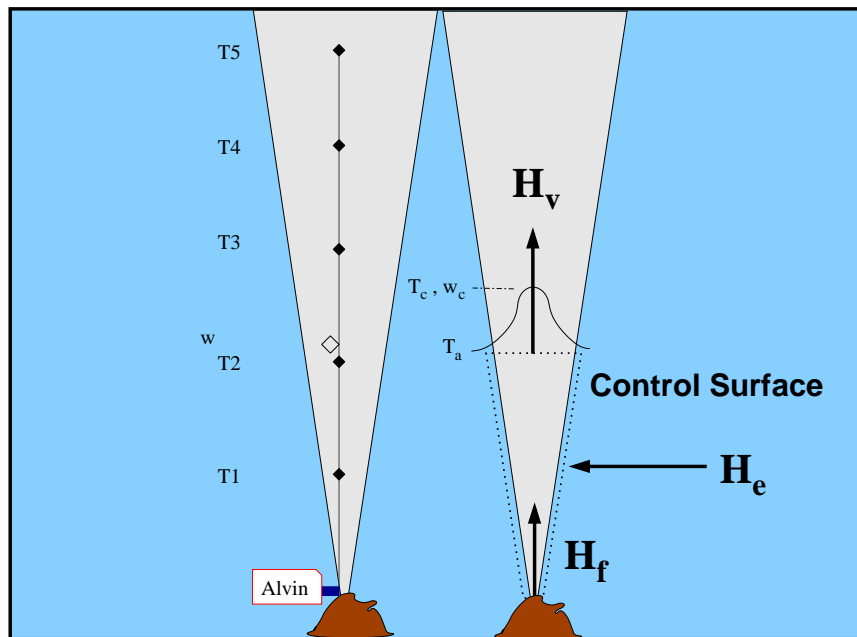
Figure 1.9: Schematic of the Bemis et al. experiment. The plume on the left contains a diagram of the array of thermistor and flow meter instruments. The plume on the right illustrates a control volume and heat fluxes associated with the source ( H_f ), the rising plume ( H_v ), and the entrained fluid ( H_e ). A Gaussian profile of mean T and w across the plume is depicted near the depth of the T2 thermistor and flow meter. Plume boundaries are drawn approximately to scale if defined by the radial distance from the centerline at which T and w become undetectable by the instruments of Bemis et al. (1993) ( \sim 4 m radius at \sim 20 m elevation).
