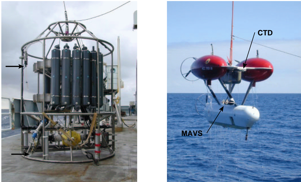
Figure 2.7: The lowered CTD package (left) and the Autonomous Benthic Explorer (right) that were utilized during the Flow Mow cruise. Note the 144 cm vertical separation of the CT sensor pairs (arrows) on the CTD package, and the relative location of CTD and MAVS on ABE.
