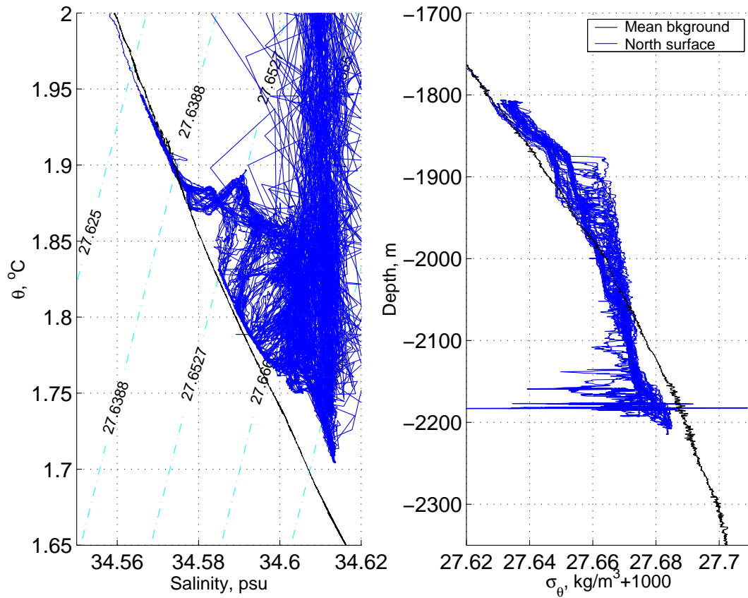
Figure 2.27: Raw 0.5 Hz data from CTD station 10, both the VOT portion along a cross-axis plane just north of the MEF, and the horizontal tow portion that passed through a buoyant plume near Hulk. Left panel shows the \theta - S trends over \sigma_\theta isopycnals. Right panel shows the \sigma_\theta depth profile. Black trace is the mean of both background stations; blue trace represents station 10 data.
