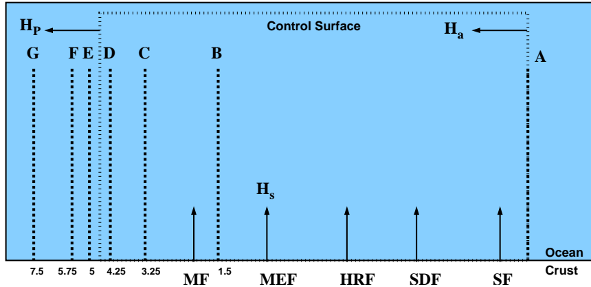
Figure 1.7: Schematic of the BAKER and MASSOTH (1987) measurement of heat flux in advected equilibrated plumes above the Endeavour segment. Approximate along-axis positions of known vent fields are depicted as source fluxes (vertical arrows) along with axis-perpendicular CTD transects (dotted lines A–G, with distance from MEF noted in km for downstream sections, B–G). Field names are abbreviated as in Figure 2.1; other annotations are consistent with Figure 1.2.
