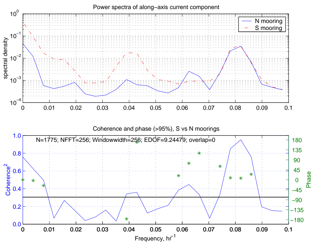
Figure 2.17: Power spectral density of the along-axis component of flow measured at the N and S moorings (top), and coherence (solid line) and phase (asterisks) between the 2 moorings (bottom). The level of 95% confidence is indicated by the horizontal line. The three significant peaks (excluding the low frequency shoulder) correspond with the diurnal, inertial, and semidiurnal periods. Positive phase means that S leads N.
