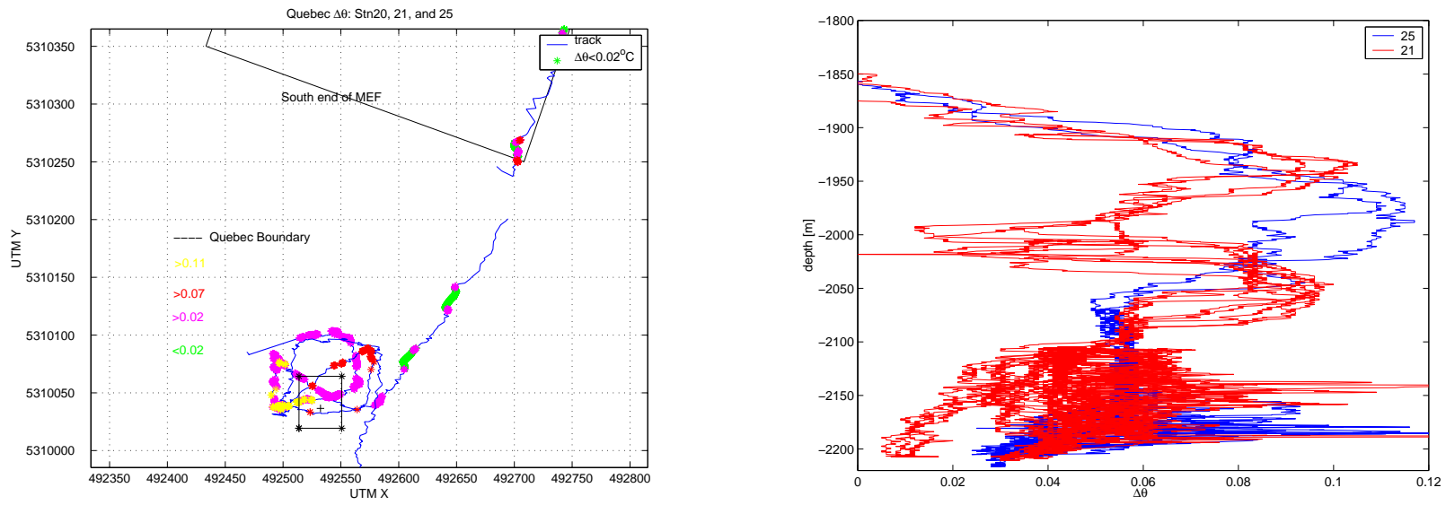
Figure 3.3: Map on left shows the CTD track during 2 VOTs around and over the Quebec diffuse flow site ( 47^{\circ}56.62'N , 129^{\circ}6.0'W ). Overlain in color are ranges of \Delta\theta encountered along the tracks; see legend for temperature ranges. Quebec coordinates, based on a 1995 Alvin dive, are delineated by the small box containing the + symbol. The southern end of the MEF is near the top of the map, along with the beginning of the track for CTD station 20, which traversed the east side of the MEF. The \Delta\theta profiles at right are derived from the 2 stations that surveyed Quebec (21 and 25).
