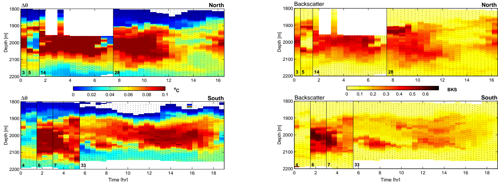
Figure 4.1: Time series of spatially and temporally averaged \Delta\theta (left) and backscatter (right) from CTD surveys of the NoMEF (upper) and SoMEF (lower) areas. Dotted black line is CTD track. Averaging bins are 1/2 hr wide and 5 m high. Vertical black lines mark temporal breaks ( \sim 1 -5 days) between stations, each of which is numbered in lower left corner. White areas have no data (or \Delta\theta < 0^\circ\text{C} ). See Figure 3.4 for additional notes and \Delta\theta detail in bottom 100 m.
