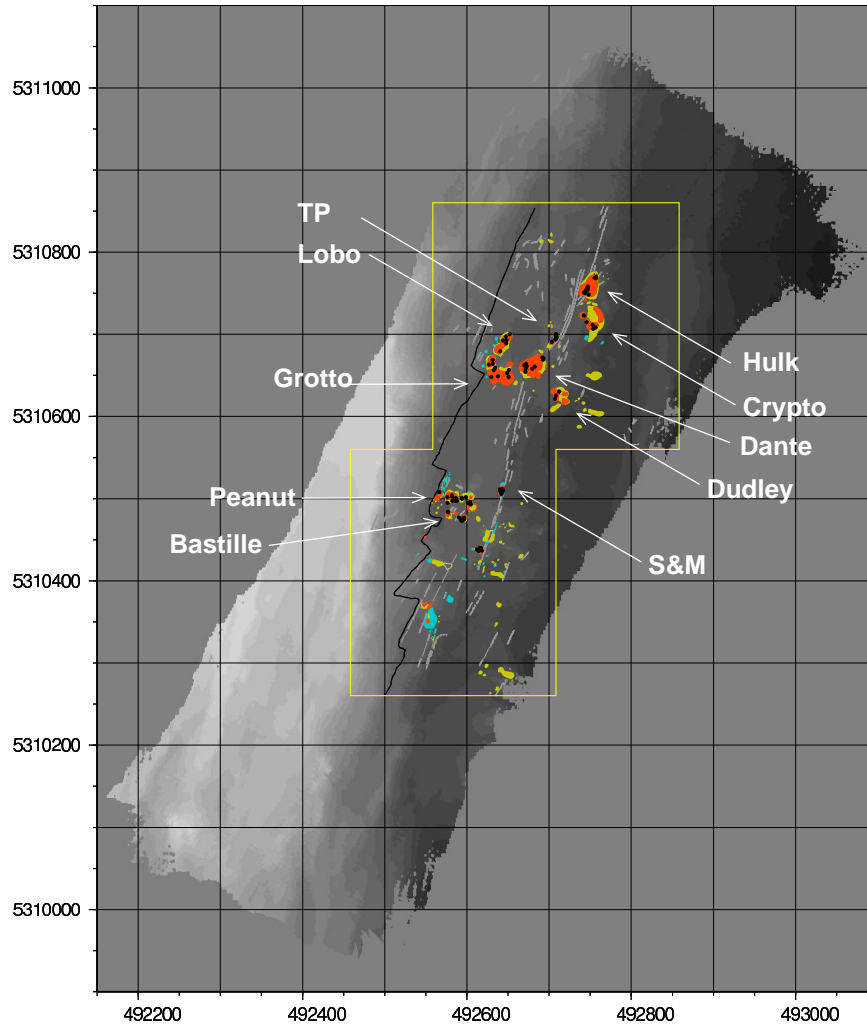
Figure 2.6: Digitized version of the geologic map of the MEF created by V. Robigou (DELANEY et al. 1992). Arrows connect names to sulfide structures that are actively venting from high B sources (black dots). Inactive sulfide structures are yellow. Areas of diffuse venting are light blue. Major fissures and faults are delineated in grey. Approximate location of contact between talus scarp and valley floor is shown by jagged black line near western edge of field.
