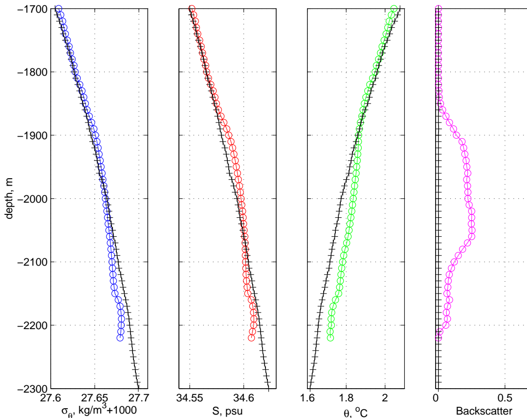
Figure 2.23: Observed profiles of mean \sigma_\theta , S , \theta , and backscatter data combined from the NoMEF and SoMEF areas, \sim 500 m north and south of the MEF. Each circle is the mean of all data within a 25 m depth bin centered at that depth. Note that the deepest 2 bins include data from the SoMEF area only.
