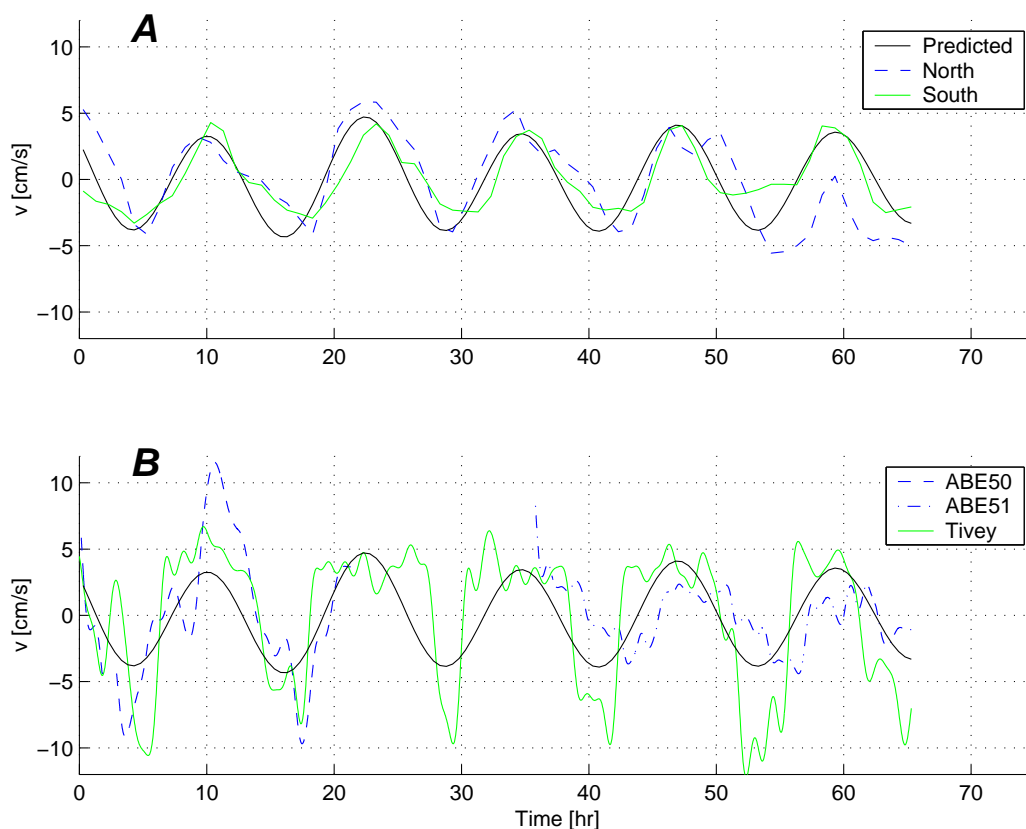
Figure 2.18: The zero-mean, along-axis component of flow measured at A) FM-N15 north of MEF (dashed blue) and FM-S50 south of MEF (solid green), and B) by ABE on the Flow Mow control surfaces (dashed blue) and by a near-bottom MAVs in the middle of the MEF (solid green). Each series covers the same period as in Figure 2.15 and is overplotted with a solid black curve: flow extrapolated to the year 2000 through harmonic analysis (H. Mofjeld, pers. comm.) using 60 days of 10 min mean data from MZ25 (Table 2.1). Time series in B) derive from: a MAVS deployed by M. Tivey \sim 0.5 mab and 40 m north of the S&M sulfide structure (Figure 2.6); a MAVS mounted on ABE during the 2 longest dives (ABE50 and ABE51). All MAVS data were smoothed with Butterworth low pass filters ( e.g. EMERY and THOMSON 2001).
