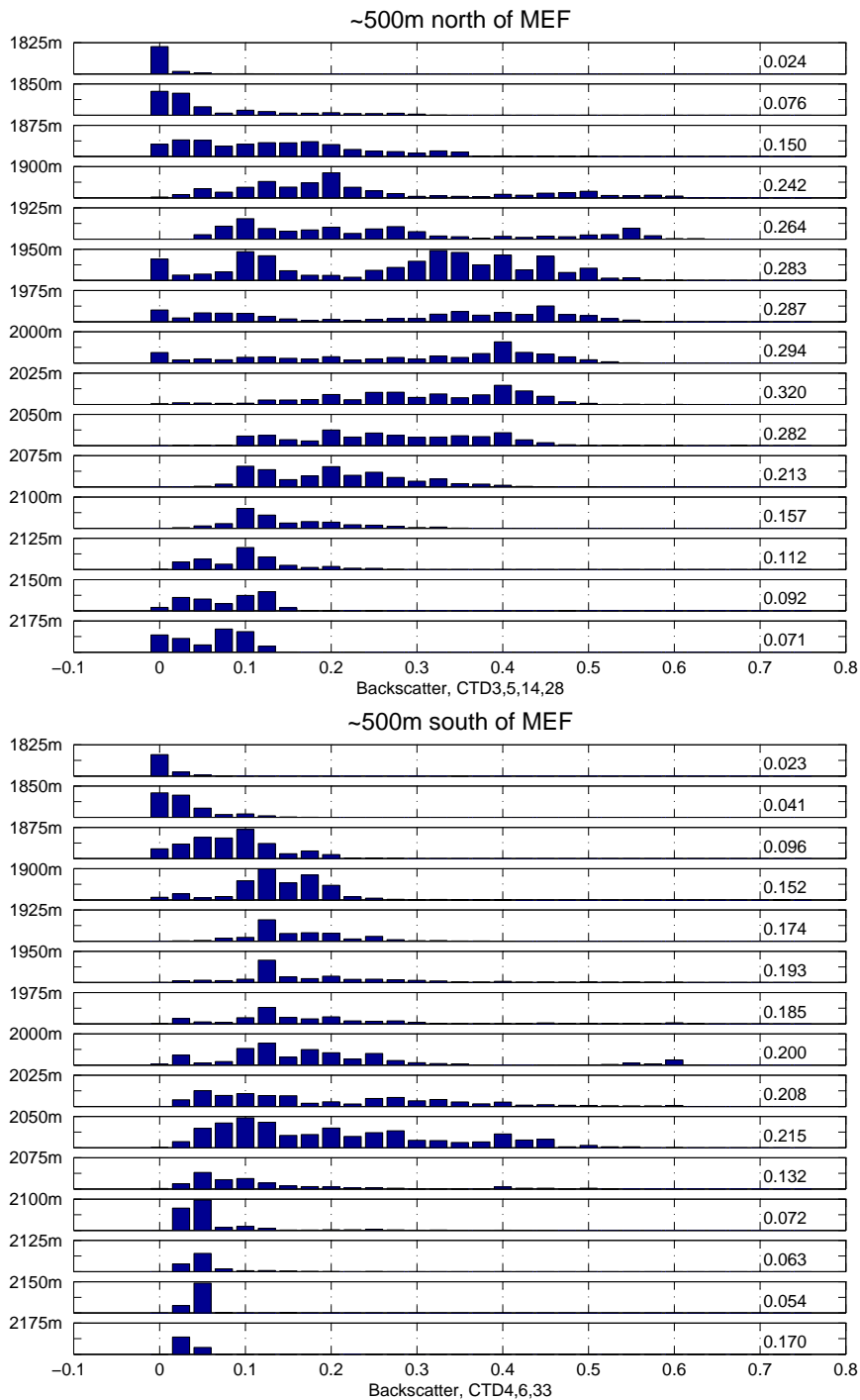
Figure 4.2: Histograms of all backscatter data from the NoMEF (upper) and SoMEF (lower) areas (Figure 2.5), except station 7, binned in depth intervals of 25 m. Mean values of distribution in each bin are listed at right.
