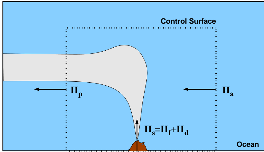
Figure 1.2: A generic control volume over a hydrothermal vent field in a steady cross flow. H_s is a source heat flux through the horizontal bottom surface. H_a is the flux of ambient heat carried by the cross flow from right to left through the vertical upstream surface. H_p is the flux through the vertical downstream surface, including ambient and plume components. Zero flux is assumed for the top surface, as well as the near and far vertical surfaces that are oriented parallel to the cross flow. H_d and H_f are the heat fluxes through diffuse and focused vents, respectively, and may generate plumes with a wide range of rise heights — not necessarily characterized accurately by the light grey schematic plume.
