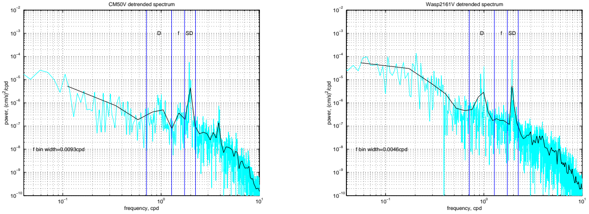
Figure 2.16: Power spectra of near-bottom v at FM-S50 (left) and FM-N15 (right). The diurnal, inertial, and semi-diurnal frequency bands are labeled D, f, and SD.
