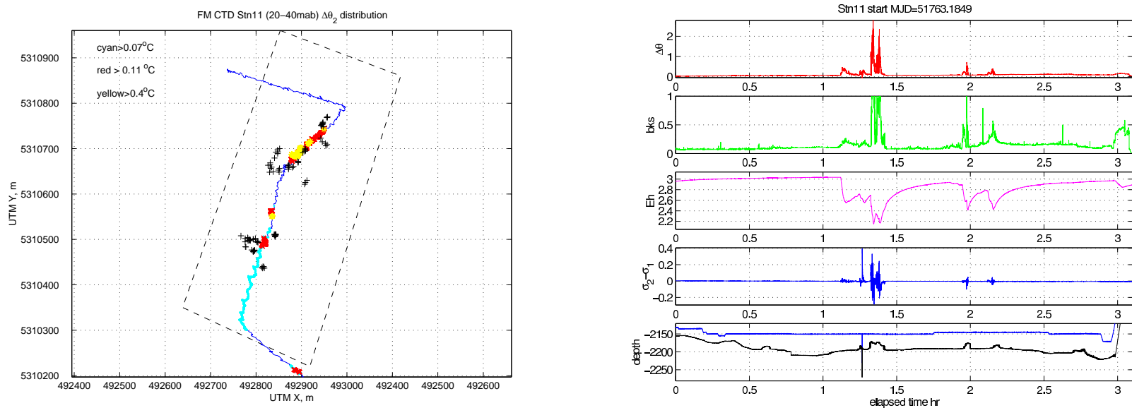
Figure 2.28: Location map and time series from horizontal tow through buoyant plumes during CTD station 11, which proceeded from north to south. Left panel symbols: dashed line is MEF control volume perimeter; each + is a known individual high B source; colored x and * symbols indicate thresholds of \Delta\theta annotated in upper left corner. Right panels (top to bottom) show time series of: (1) \Delta\theta , (2) backscatter, “bks,” (3) Redox potential, “Eh” (values decrease in reducing solutions, K. Nakamura, pers. comm.), (4) difference in potential density observed at upper and lower CT pairs ( c.f. Figure 2.7), indicating fluid instability (VEIRS et al. 1999), and (5) depth and bottom traces (based on CTD depth and altimeter readings).
