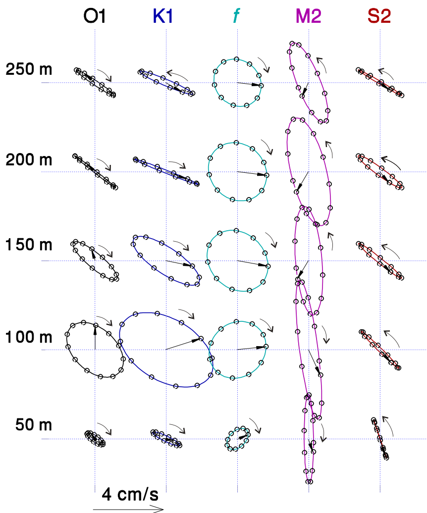
Figure 2.14: Current ellipses and vectors at 5 depths on the southern mooring for the main tidal frequency bands ( O_1 , K_1 , M_2 , S_2 ) and the inertial frequency band ( f ). Meter elevation is noted on the left in meters above bottom. Current vectors indicate a reference time to illustrate relative phase. Small circles denote hourly mean values for current vectors. Outer arrows show direction of vector rotation. Along-axis ( 20^\circ True) direction is upward. Figure used with permission from THOMSON et al. (2003), courtesy R. Thomson.
