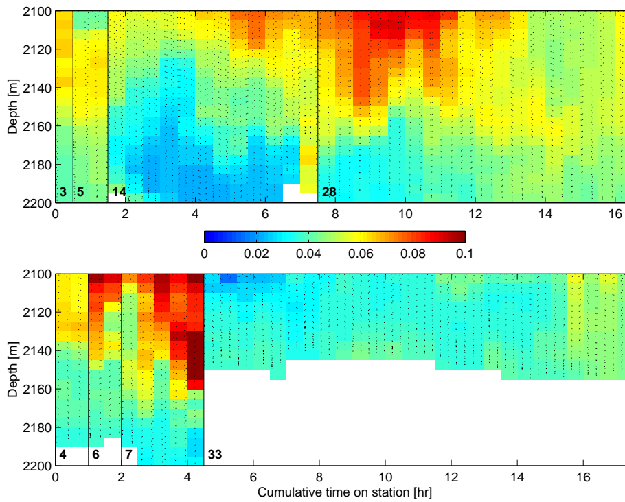
Figure 3.4: Time series \Delta\theta from vertical CTD casts in the NoMEF area (top panel) and SoMEF area (bottom panel). Before plotting, data were averaged in vertical bins 5 m high and 1/2 hr wide. White areas contain no data. Dotted black line represents CTD depth history. Vertical black lines mark temporal breaks of \sim 1 -5 days between stations, each of which is numbered in lower left corner. Station 33 does not extend below 2155 m because it was located west of stations 4, 6, and 7, where the western scarp shoals to \sim 2160 m (see dual SoMEF locations, Figure 2.1). For additional context, see Figure 4.1.
