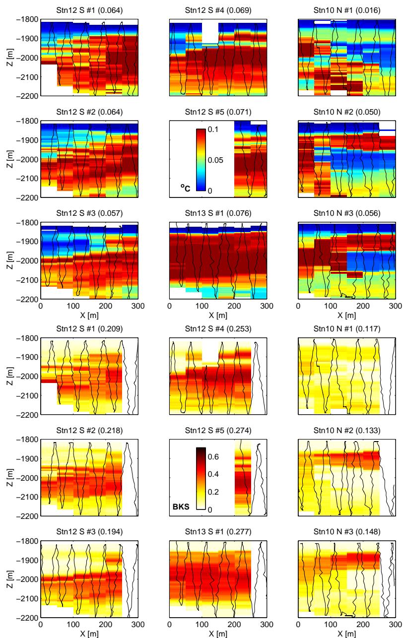
Figure 4.3: \Delta\theta (upper panels) and backscatter (lower panels) distribution on north and south MEF control surfaces: 1800–2200 m. Left 2 columns depict surveys of south surface; right column depicts surveys of north surface. Each survey is labeled with: its station number; its order in the sequence of surfaces surveyed during that station ( e.g. 12#3 is the 3rd surface observed during station 12); and the mean value of \Delta\theta or backscatter (noted parenthetically). White areas have no data (or \Delta\theta < 0 ); black lines are CTD track. Central color scales give values.
