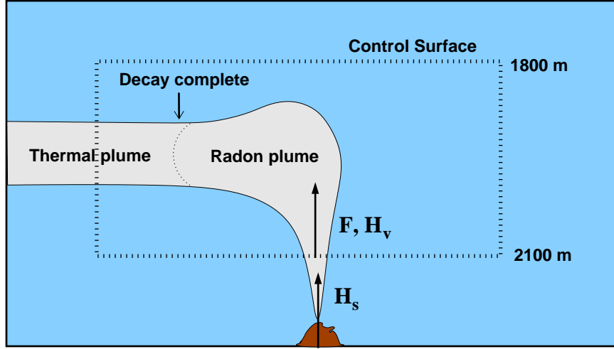
Figure 1.8: Schematic of the ROSENBERG et al. (1988) measurement of radon flux F and heat flux H_v through the 2100 m isobath near the MEF. Note that H_s does not necessarily equal H_v .
