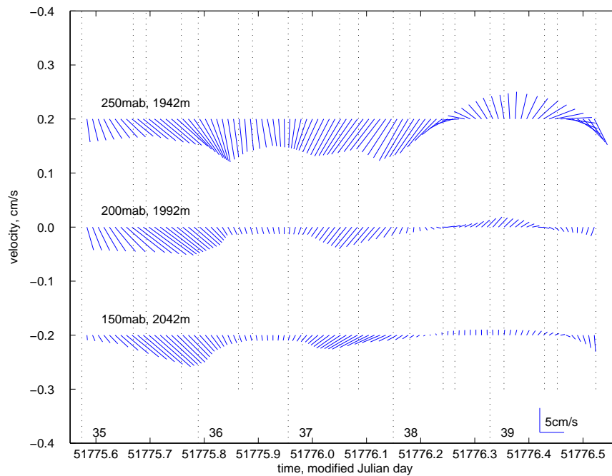
Figure 4.5: Time series of quarter-hourly mean currents observed during 5 circuits of the upper control volume at depths of 1942 m (top), 1992 m (middle), 2042 m (bottom) on the southern mooring (FM-S, Table 2.1). Vertical dashed lines show the time at which the survey of each surface began during stations 35–39 (see Figure 4.4). Each station label is just to right of time at which first surface survey began for each station.
