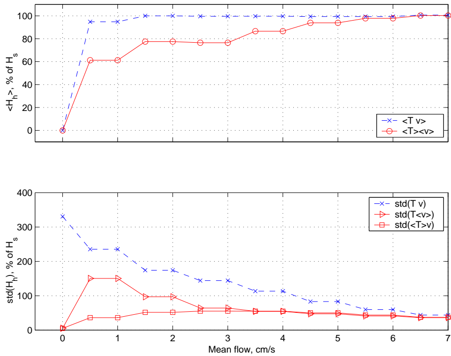
Figure 3.9: Means and standard deviations (std) of net horizontal flux ( H_h ) series from puff model simulations in which mean flow of 0–7 cm/s were added to characteristic oscillations. Statistics are expressed as percentage of source heat flux ( H_s ). Lower panel shows standard deviations of the 3 types of net heat flux series : instantaneous ( T v ), velocity-averaged ( T \langle v \rangle ), and temperature-averaged ( \langle T \rangle v ). Upper panel shows the mean of the instantaneous series ( \langle T v \rangle ) and either averaged series ( \langle T \rangle \langle v \rangle ) for each mean flow.
