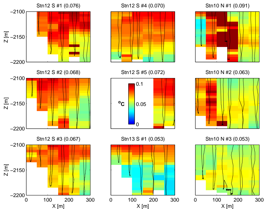
Figure 3.2: Isohaline potential temperature anomaly \Delta\theta on south (left 2 columns) and north (right column) control surfaces during CTD stations 10, 12, and 13. Title above each panel indicates: CTD station number; south (S) or north (N) surface; order (#) in sequence of surface surveys during each station; mean of all bins (noted parenthetically). Station 12 began \sim 3.8 hr after station 10 ended, and station 13 began \sim 14.2 hr after the end of station 12; sequential surveys during each station are temporally contiguous. Bottoms of successive vertical oscillations are spaced \sim 20 min apart; surfaces were surveyed in \sim 80 – 100 min. Black line represents CTD track. Averaging bins are 100 m wide and 5 m high. White areas have no data.
