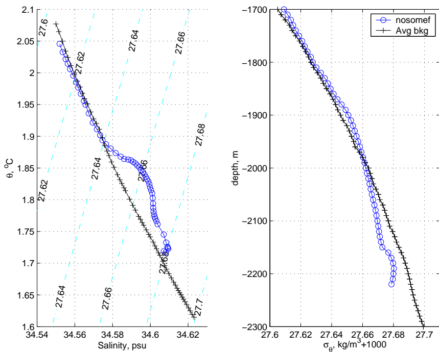
Figure 2.25: Mean \theta - S and \sigma_\theta profile based on data combined from NoMEF and SoMEF areas and averaged in 10 m depth bins. The equilibration depth, 1980 m, is associated with the \sigma_\theta = 27.66 \text{ kg/m}^3 isopycnal. Note that isopycnals in the \theta - S plot are only parallel to isobaths (lines connecting bins of the same depth) at the equilibration density, 27.66 \text{ kg/m}^3 ; that is, at all depths greater than \sim 1800 m the mean isopycnal surfaces are sloped above and below 1980 m.
