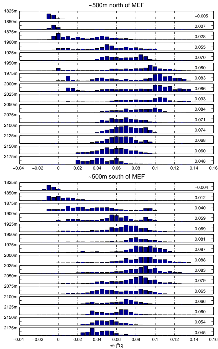
Figure 3.6: Stacked histograms of depth-binned \Delta\theta observed north (upper) and south (lower) of the MEF. Depth range of each bin is 25 m and upper extent of each bin is noted on the left axis. For reference, the nearby ridge crests have a mean depth of \sim 2100 – 2125 m. \Delta\theta for each distribution is tabulated at right. North data is from CTD stations 3, 5, 10, 14, and 28, and ABE dives 45, 46, and 50; south data is from CTD stations 4, 6, 7, 12, 13, and 33, and ABE dives 45, 46, 50.
