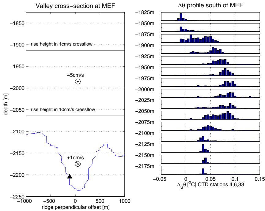
Figure 2.2: Axial valley relief and current shear relative to plume rise heights. The left panel shows an axis-perpendicular cross-section of the Endeavour segment Hydrosweep bathymetry (D. Kelley, 1996), with the location of the MEF indicated by a black triangle. The mean flow within and above the axial valley is indicated, along with the range of rise heights expected in cross flows of 1–10 cm/s. The right panel shows stacked histograms of temperature anomaly data that were acquired during a 14 hr CTD station \sim 500 m south the MEF and subsequently grouped into 25 m depth bins.
