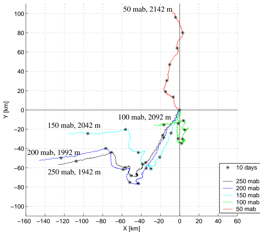
Figure 2.11: Progressive vector diagrams for 5 current meters on mooring FM-S (Table 2.1). Entire 74 day record is used with asterisks indicating 10 day intervals. Relative to these intervals, the 17 day Flow Mow cruise period (Julian day 217–234) was from day 7 to day 24.
