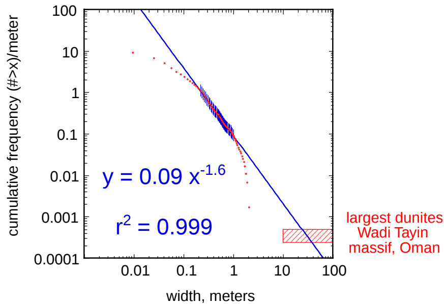
Figure 7. Dunite width in Ball outcrop (Figure 2) versus cumulative frequency (number of observations with width greater than x ). Data for dunite width greater than 0.2 m and less than 1 m, where sampling density is high, were fit to derive a power law relationship, which was then extrapolated to the sizes of the largest dunites in the mantle section of the Oman ophiolite. The small-scale data from the Ingalls ophiolite are roughly consistent with the frequency of large dunites in Oman.
