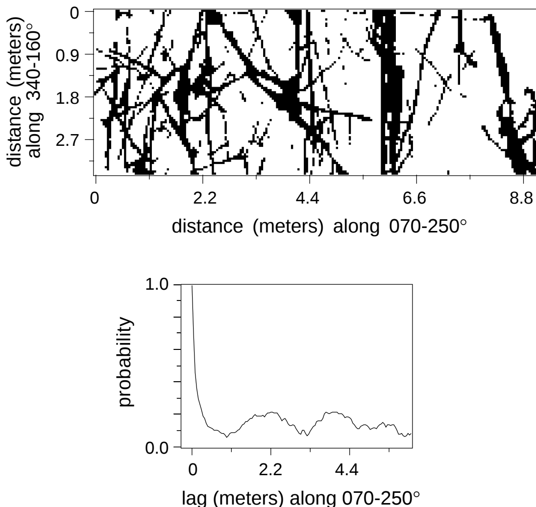
Figure 4. Lower-resolution image from the Ball outcrop (Figure 2), and results of two-dimensional autocorrelation analysis of this image. Note that for this analysis, eroded areas which we interpreted as dunites were treated as dunite outcrop areas.
