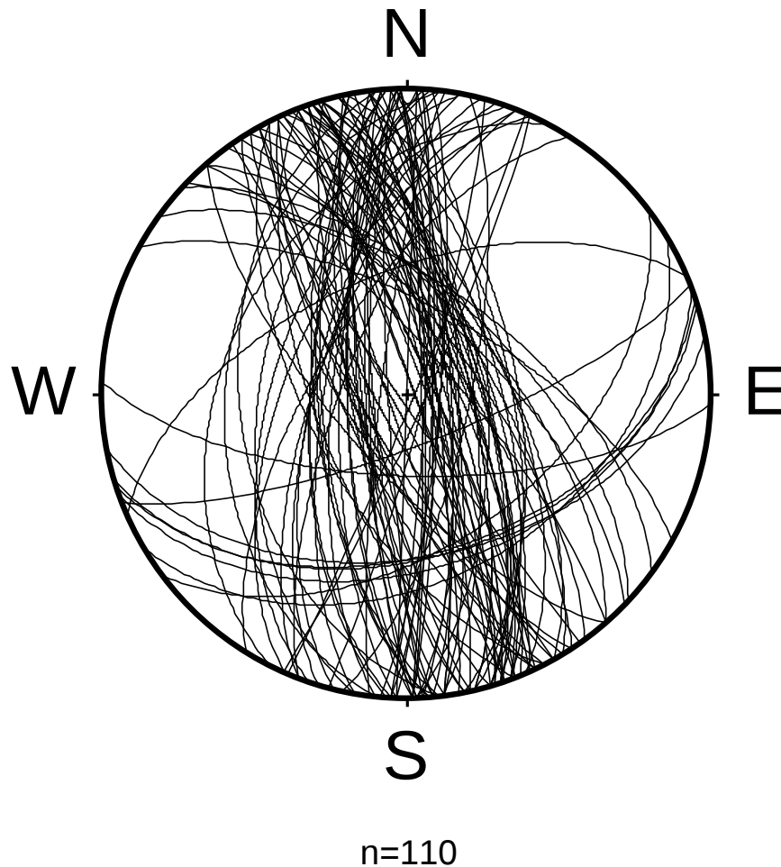
Figure 1. Lower hemisphere projection of orientation of dunites within residual mantle peridotite (harzburgite) in Bean Creek outcrops of the Ingalls ophiolite. Most dunites are approximately perpendicular to the surfaces of outcrops dipping 25^{\circ}\text{S} , which were mapped for this study.
