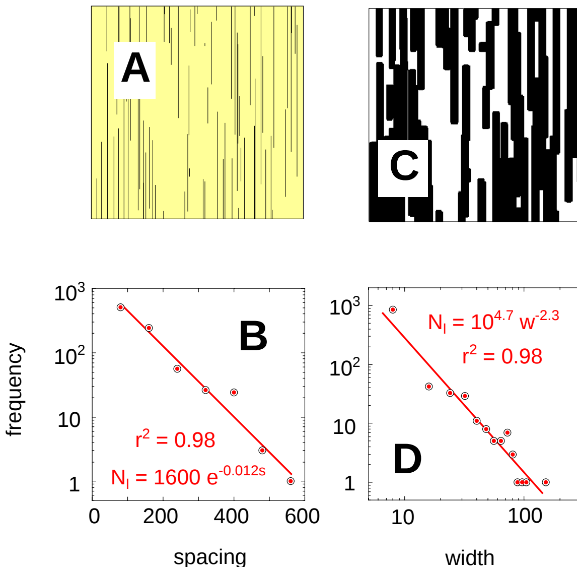
Figure 6. Results of a simple model of reaction zones around parallel cracks. (A and B) Randomly spaced, parallel cracks, and their spacing statistics; (C) reaction zone distribution after 15× widening of initial, 1 pixel wide “reaction zones”; (D) size/frequency statistics when reaction zones occupy 80% of a model space larger than Figure 6C.
