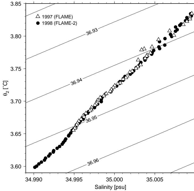
Figure 3: \theta_2/S comparison of deep 1997 and 1998 profiles from the deep basin near 36.25^\circ\text{N} ; the 1998 profile is truncated at 3200 m, the maximum depth of the 1997 profile; \sigma_2 contour interval is 0.01.
