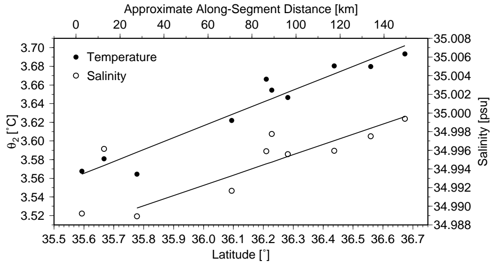
Figure 5: Scatter plots and linear regressions of the rift-valley temperatures and salinities at 2550m; the two southernmost profiles contain salinity inversions and are not used for the salinity-gradient calculation; the regression coefficients ( \pm 1\sigma ) and RMS errors are 1.0(\pm 0.1) \times 10^{-3} \text{C}\cdot\text{km}^{-1} and 1.2 \times 10^{-2} \text{C} , and 8.5(\pm 1.7) \times 10^{-5} \text{psu}\cdot\text{km}^{-1} and 1.4 \times 10^{-3} \text{psu} , respectively.
