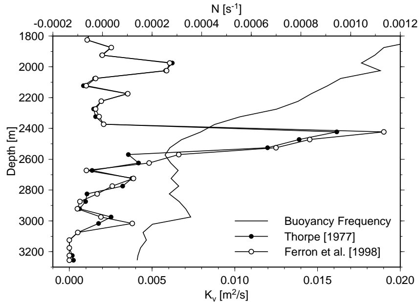
Figure 12: Ensemble-averaged rift-valley buoyancy-frequency and diffusivity estimates from Thorpe displacements using two different methods to account for the instrument noise ( 2 \times 10^{-4} \text{ }^\circ\text{C} ).
