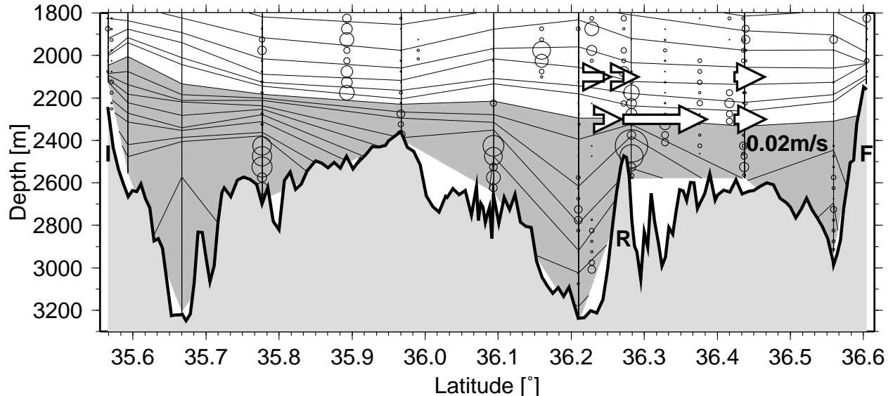
Figure 10: Rift-valley density section (contours), flow speeds (the lengths of the arrows, measured from the bases of the stems to the tips, show mean along-valley velocities observed during the final week of current-meter deployment, c.f. figure 7), and diffusivity estimates from overturning scales (“bubbles,” c.f. section 6); the path of of the along-segment bathymetry is shown in figure 1; see text for station selection and sill labelling; density contours are the same as in figure 6; the shaded area indicates water with \sigma_2 \geq 36.9449 .
