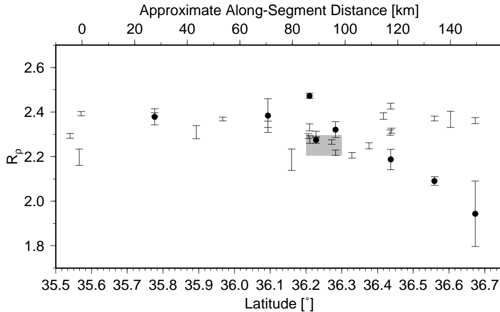
Figure 4: Rift-valley stability ratios; upper-layer values (2050–2300 m) are shown as unmarked error bars; lower-layer values (below 2300 m) are marked with bullets; grey area indicates 1997 CTD-yoyo observations (see text).
