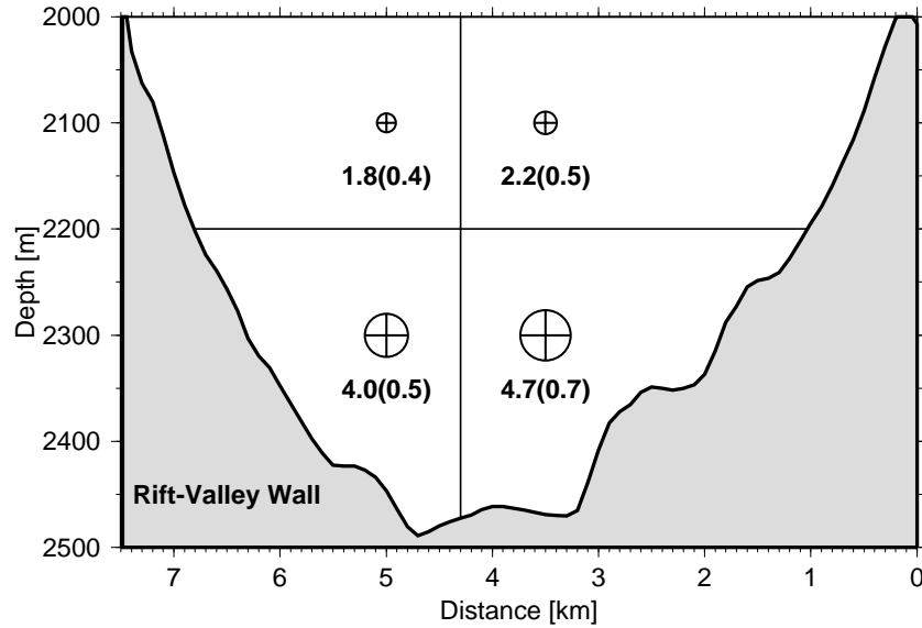
Figure 8: Cross-valley section on the sill near 36.25^\circ\text{N} (straight lines in figure 7) and location of the current meters projected onto the section (crossed circles); distance is measured from SE to NW; straight lines indicate subdivision into quadrants for transport calculations. The diameter of the current-meter symbols is proportional to the mean flow speeds normal to the section; in addition to the mean values, the uncertainties determined from the spectral properties of the flow ( Flierl and McWilliams, 1978 ) are listed in parenthesis below each current-meter; units are 10^{-2} \text{ m}\cdot\text{s}^{-1} .
