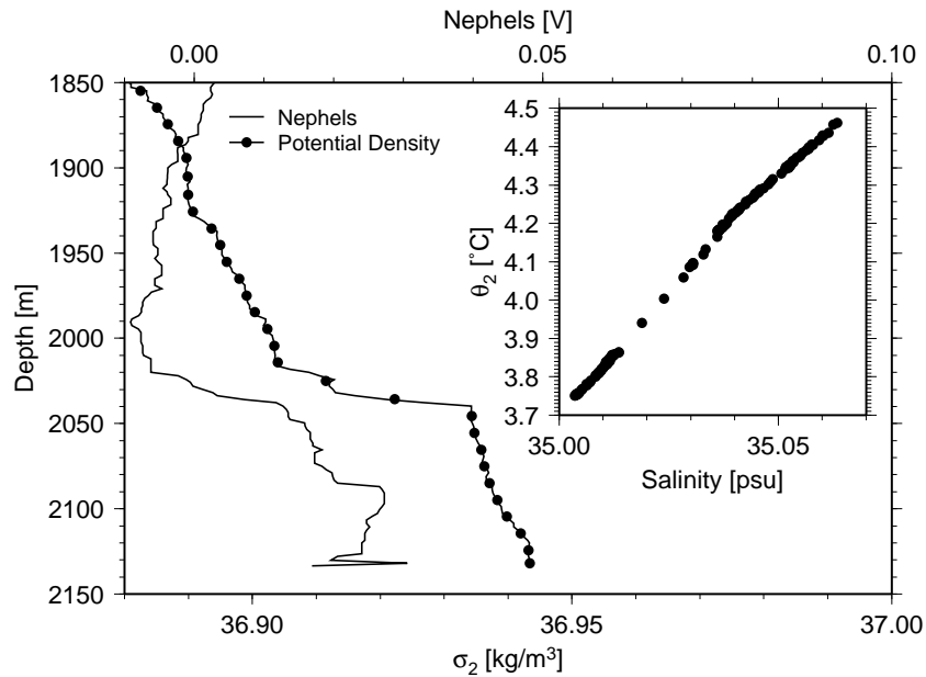
Figure 11: Hydrographic and light-scattering profiles on sill “F” connecting the AMAR and FAMOUS segments; in the main panel the potential density and nephelometry profiles are plotted; the inset shows the corresponding \theta_2/S properties.
