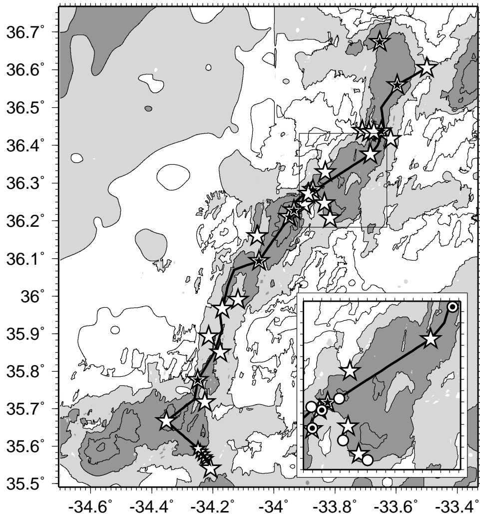
Figure 1: AMAR bathymetry (mosaic of the data sets of Needham et al. (1992) and of Smith and Sandwell (1997), version 6.2), CTD stations (stars), and current-meter moorings (circles, inset only); dark shaded regions are deeper than 2500 m, lightly shaded regions are 2000–2500 m, and unshaded regions are less than 2000 m deep; contour interval is 500 m. The small stars near 35.55°N/34.2°W show the bottom turning points of a CTD tow-yo (figure 6); black stars with white borders indicate profiles with linear \theta_2/S characteristics extending below 2550 m (section 3b.). The heavy line (main panel and inset) and the moorings marked with bullets (inset only) indicate the path of the bathymetry and the current meters shown in figure 10. The location of the inset is indicated by the rectangle in the main panel.
