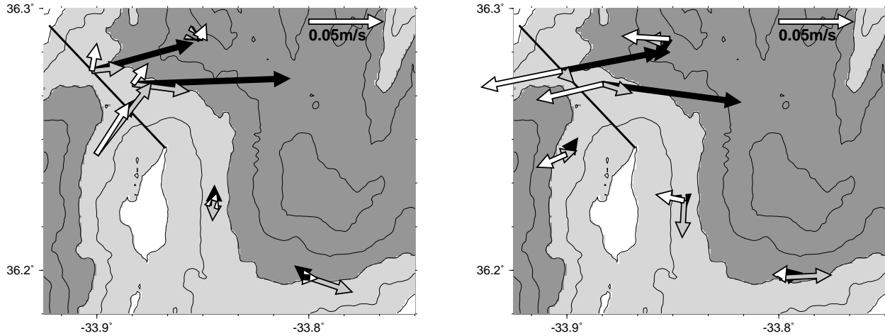
Figure 7: Average current-meter velocities in the vicinity of the sill connecting the AMAR and the South AMAR segments recorded during the first (left panel) and the last (right panel) weeks of mooring deployment; shading of the arrows is determined by the instrument depths with black, gray and white indicating 2300 m, 2100 m and 1800 m, respectively; bathymetric shading is the same as in figure 1; contour interval is 250 m. The solid along-sill lines indicate the location of the cross-valley section used to calculate the along-segment transport, c.f. figure 8.
