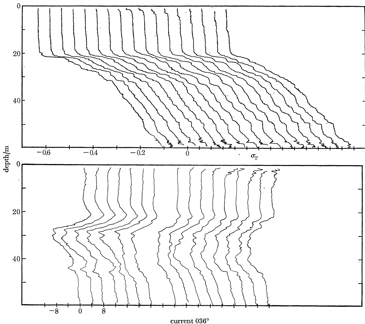
FIGURE 21. Profiles of density ( \sigma_T ) and current along the Loch in direction 036^\circ on 24 September. The profiles were made at intervals of approximately 15.3 min. There was a fault in the eighth velocity profile and it is omitted.
