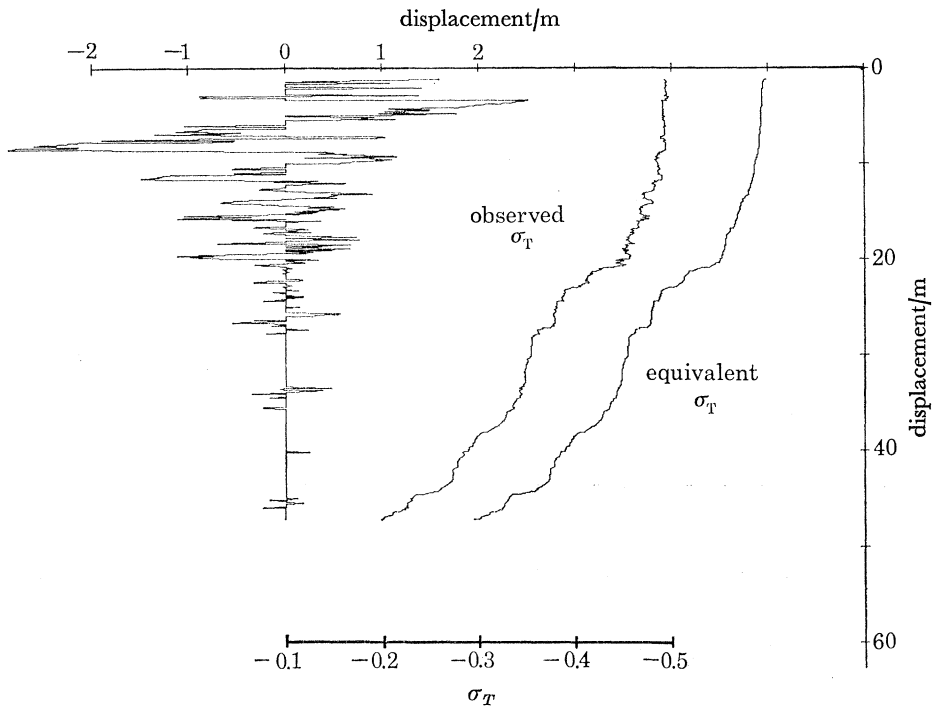
FIGURE 26. The 22nd profile of density ( \sigma_T ) on 28 September as observed, the 'equivalent' stable profile moved 0.1\sigma_T units to the right, and the displacements needed to produce the stable profile from that observed, as explained in §3.1.
